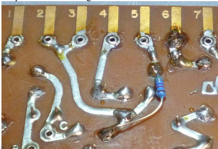
Figure 6-Final step of R30 installation in those cases where holes don't already exist on the PCB
