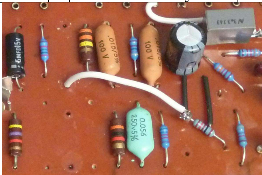
Figure 3-Detail of R2-C3-white-wire connection
