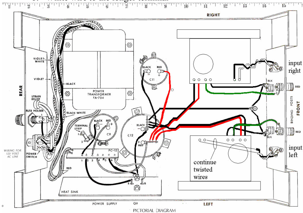
PICTORIAL DIAGRAM Figure 21-completed wiring
