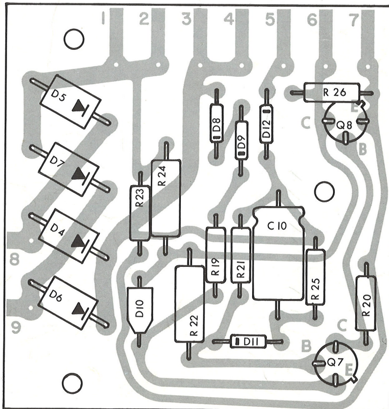
POWER SUPPLY CIRCUIT BOARD
