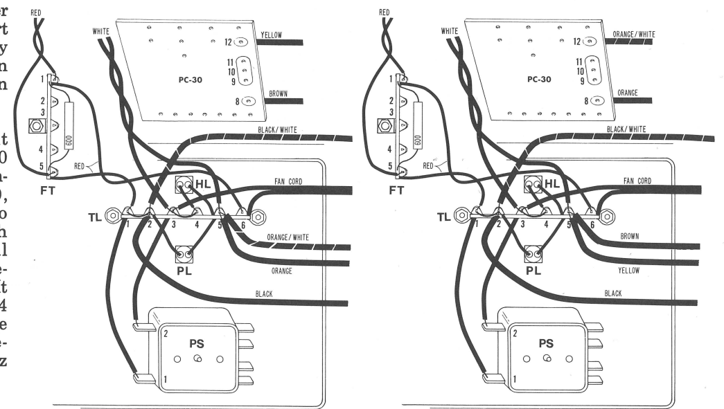
120 VAC
