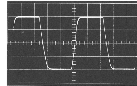
20 KHz, 200 watts
