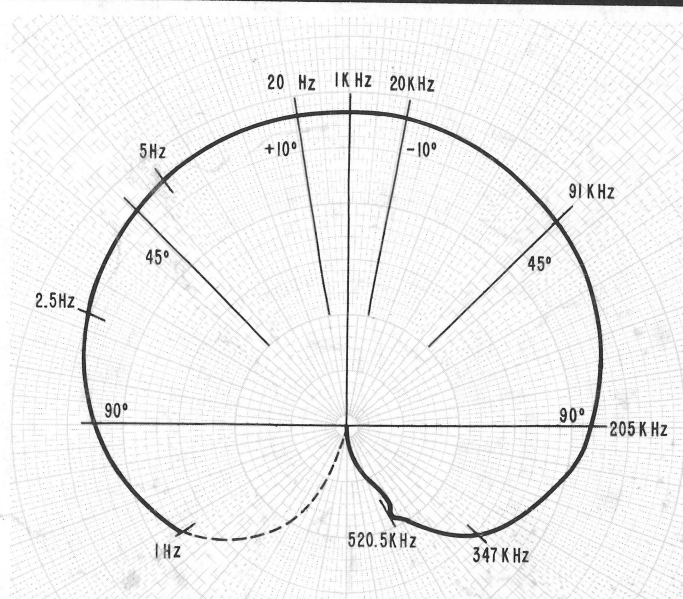
Gain-Phase Relationship
