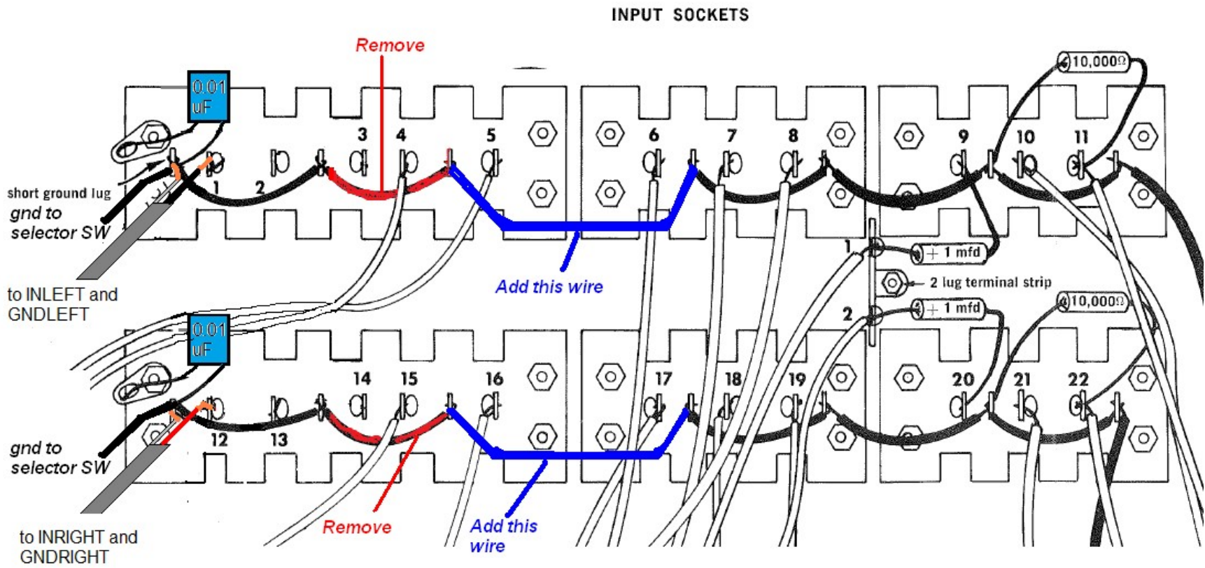
Figure 9-Back Panel Re-wiring
