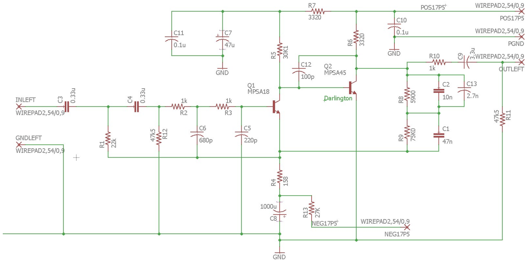
Figure 10-Phono Preamp Schematic Page 1
