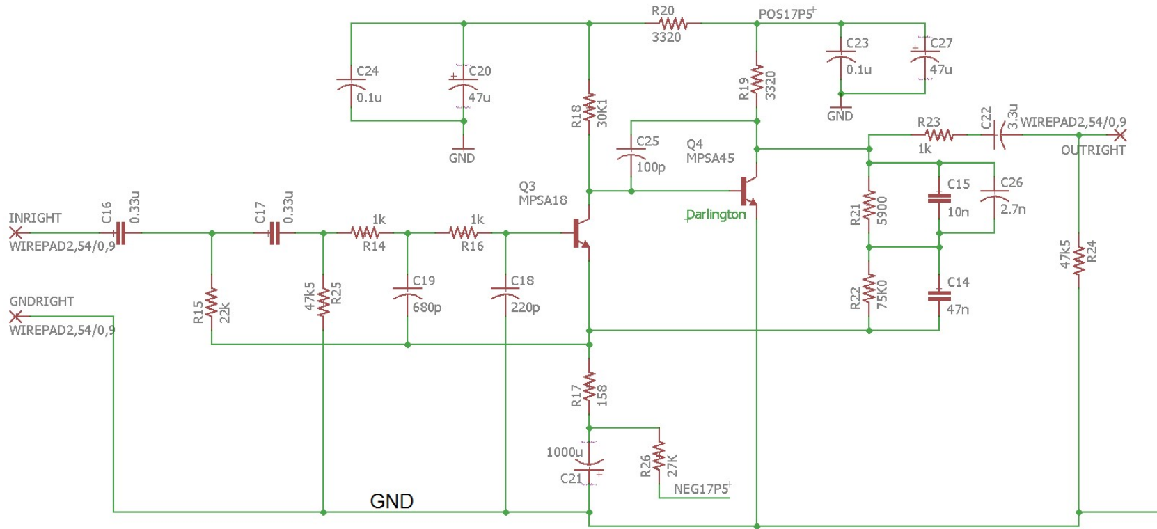
Figure 11-Phono Preamp Schematic Page 2
