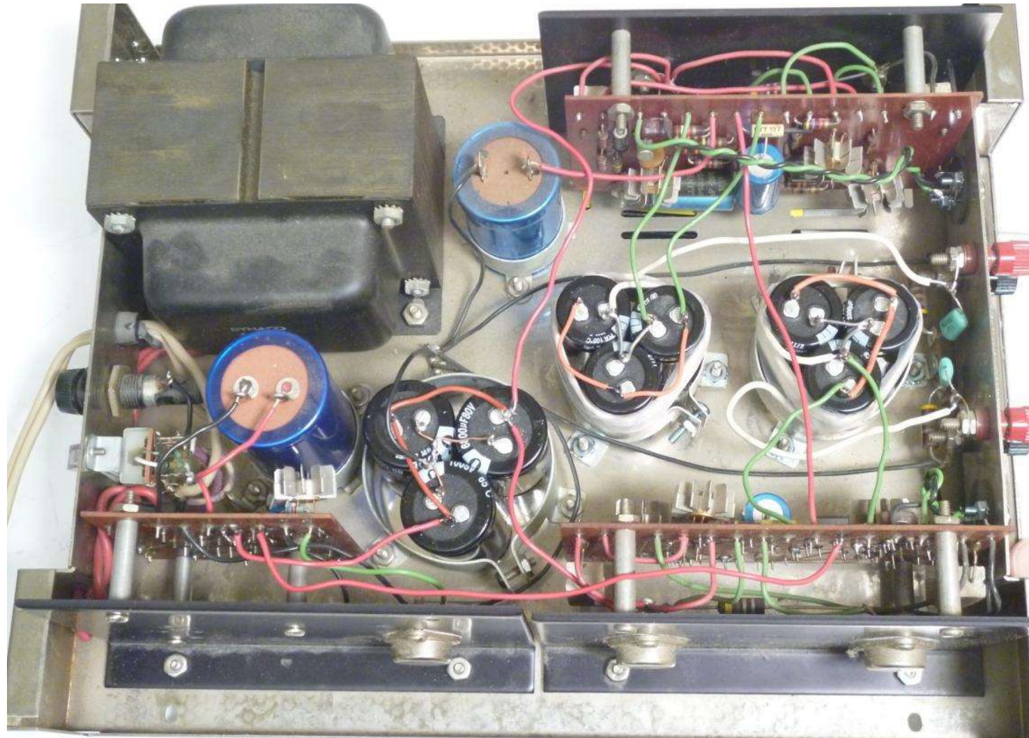
Figure 13-Completed wiring
