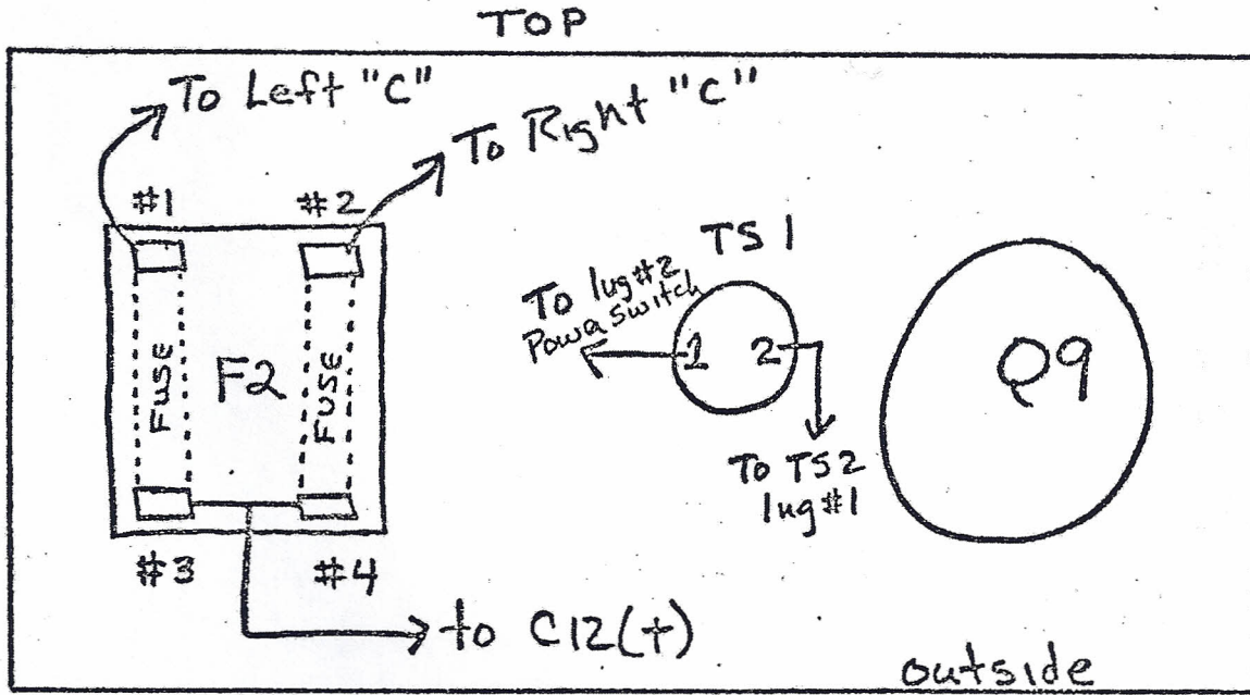
DIAGRAM A Power Supply Heat Sink
